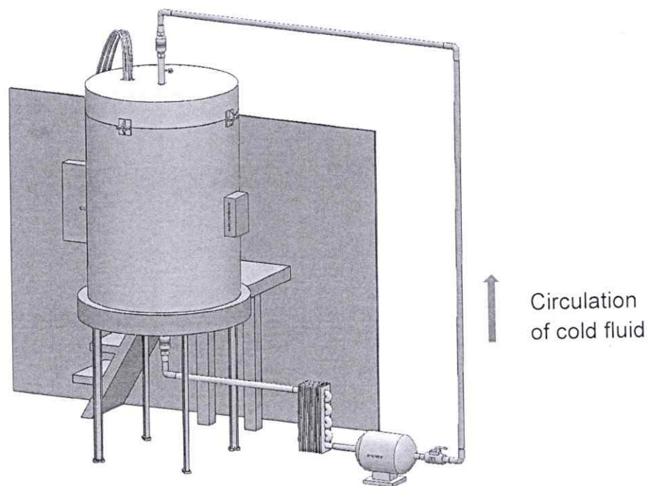
Fig1: Schematic Layout of Thermal Autofrettage Plant
